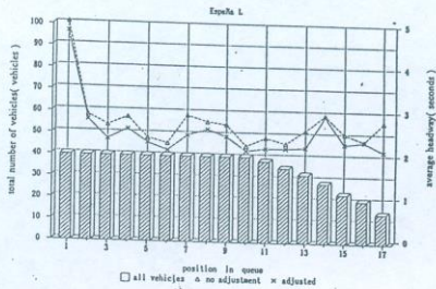
FIGURE 4 - a. Variation of average headway with and without adjustments with respect to vehicle composition in the España sample
