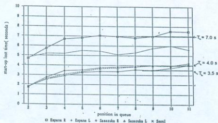
FIGURE 9. Plot of cumulative start-up lost time of vehicles
