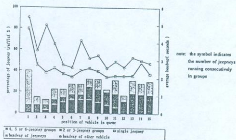
FIGURE 10. Variation of jeepney traffic, headway and grouping behavior
