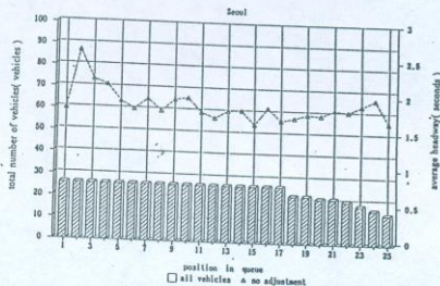
FIGURE 4 - c. Variation of average headway with and without adjustments with respect to vehicle composition in the Seoul sample
