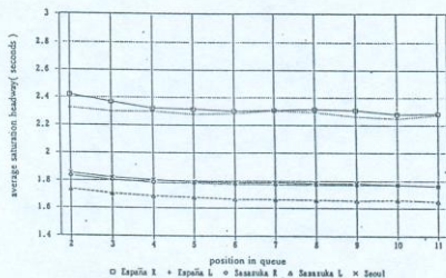
FIGURE 5. Graph of saturation headway of each position in queue
