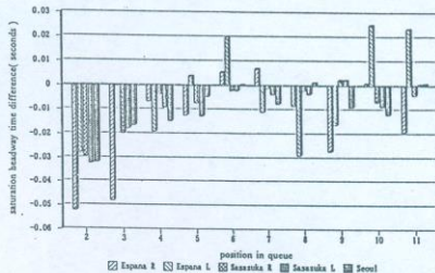
FIGURE 6. Graph of saturation headway time difference
