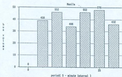
FIGURE 13. Five-minute bus flows in Metropolitan Manila
