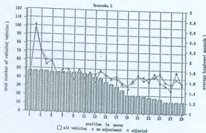
FIGURE 4 - b. Variation of average headway with and without adjustments with respect to vehicle composition in the Sasazuka sample
