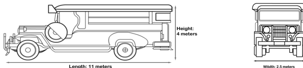
Figure 1. Vehicle Length and Height Regulations
