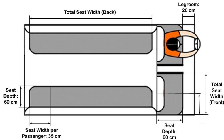
Figure 2. Minimum Seat Depth and Seat Width Regulations
