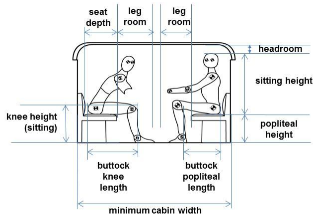
Figure 4. Passenger Cabin Dimensions
