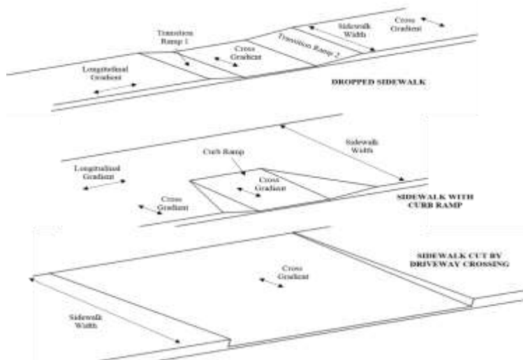
Figure 4. Types of Sidewalks and Its Components (Not to Scale)
