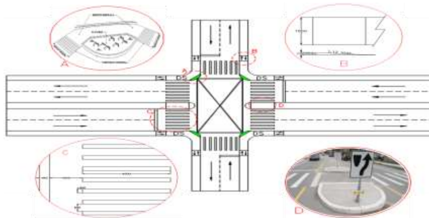
Figure 11. Sample Recommended Facilities Layout
