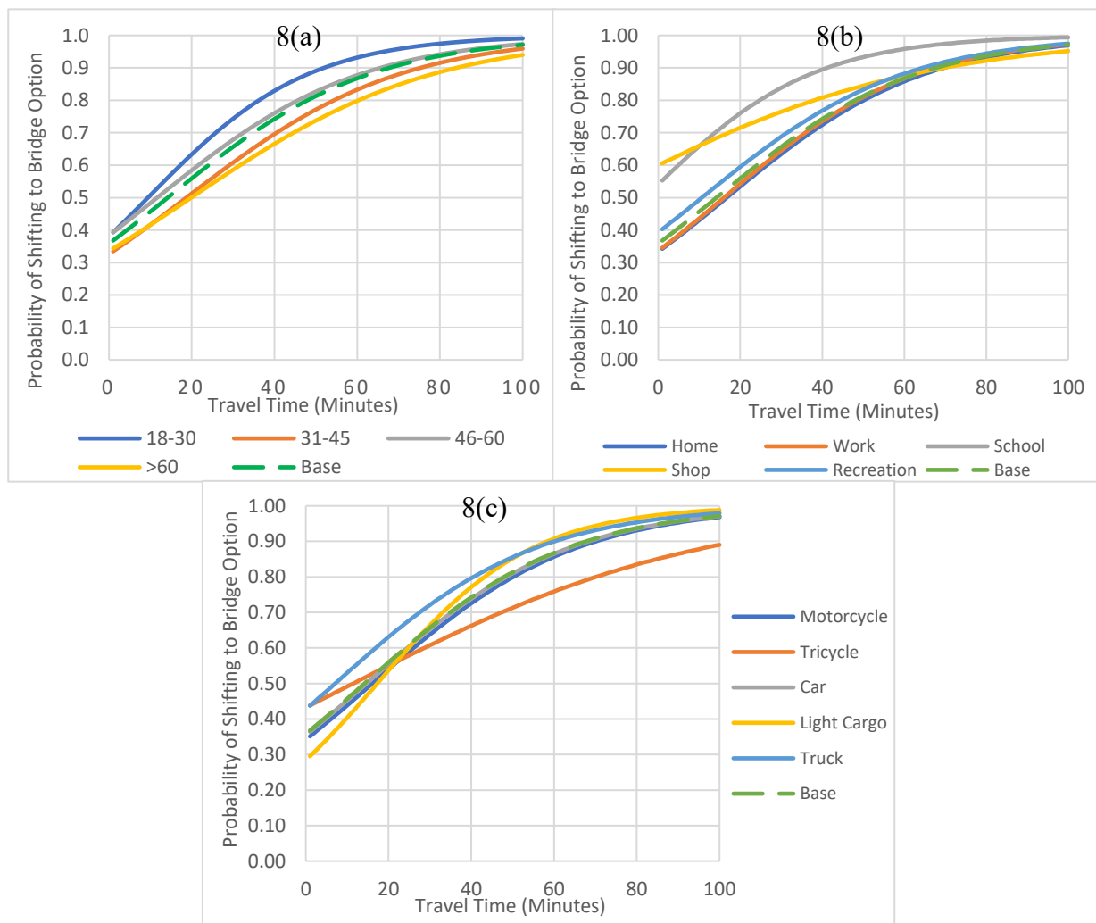
Figure 8(a). Vehicle Model - Probability curves based on travel time by age group (TOP LEFT)
